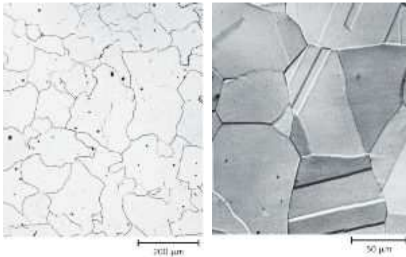
(a) Ferrite Microstructure (b) Austenite Microstructure
