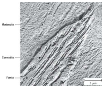
Figure 56. Image of Bainite Microstructure [3].
